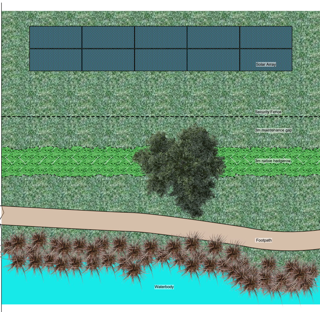
Plan View
